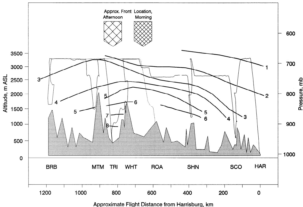
Fig. 9. Atmospheric NO y concentration contours (ppbv) derived from measurements aboard the aircraft, as in Figure 4.
