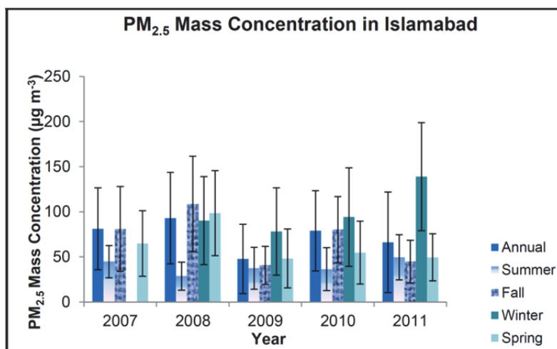
Fig. 2(a). Annual and Seasonal Average \text{PM}_{2.5} Mass Concentration ( \mu\text{g}/\text{m}^3 ) in Islamabad during 2007–2011 ( \pm 1 standard deviation is also shown in the figure).
