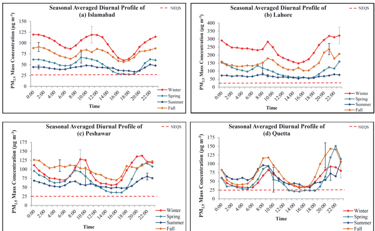
Fig. 4. Seasonal Averaged Diurnal Profile of PM_{2.5} Mass Concentration in (a) Islamabad; (b) Lahore; (c) Peshawar; and (d) Quetta ( \pm 1 standard deviation is also shown in the figure).
