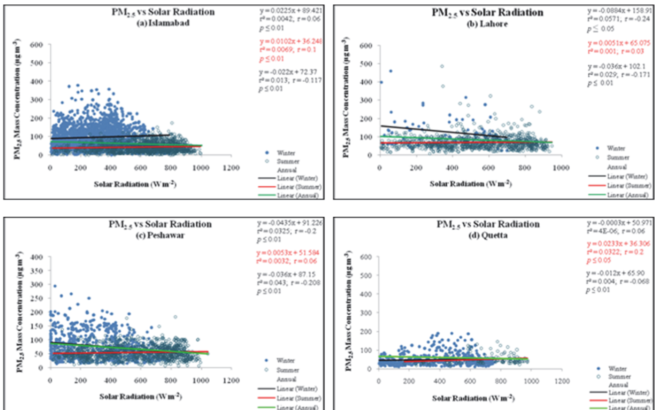
Fig. 6. Effect of Solar Radiation on PM_{2.5} Mass Concentration ( \mu g/m^3 ) during 2007–2011 in (a) Islamabad; (b) Lahore; (c) Peshawar; and (d) Quetta.
