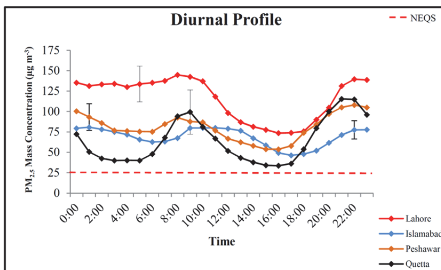
Fig. 3. Integrated Average Diurnal Profile of \text{PM}_{2.5} Mass Concentration ( \mu\text{g}/\text{m}^3 ) in Islamabad, Lahore, Peshawar and Quetta for 2007–2011 ( \pm 1 standard deviation is also shown in the figure).
