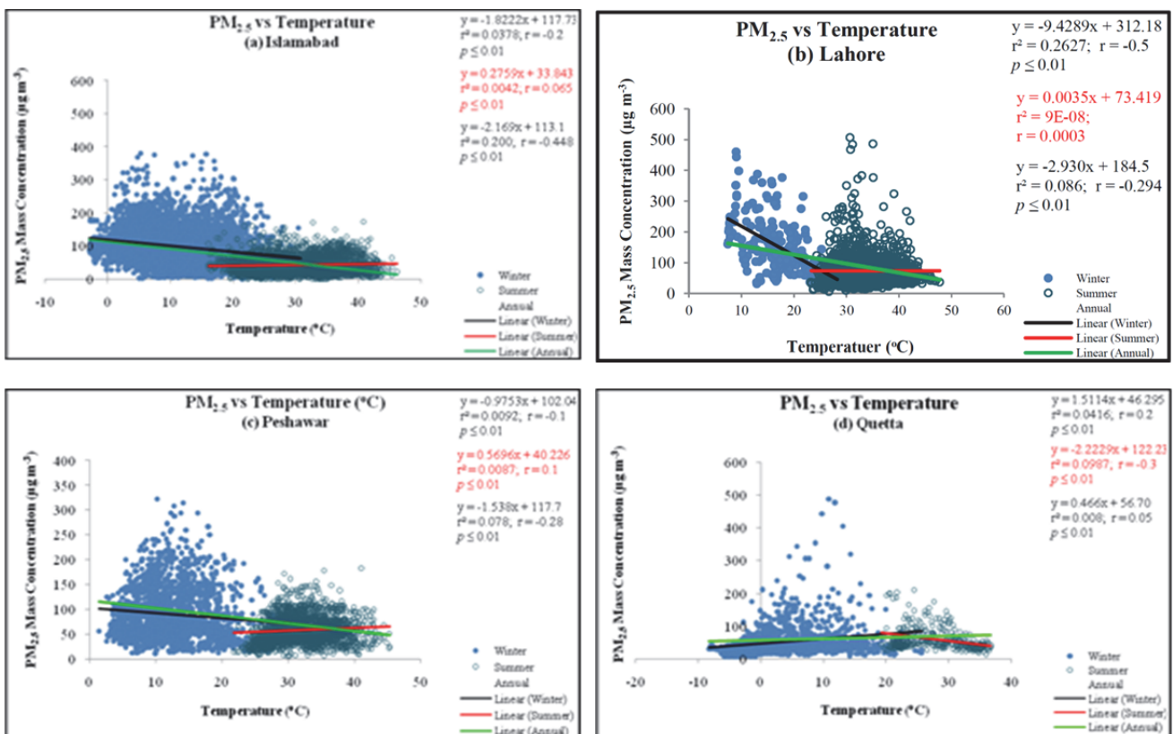
Fig. 5. Effect of Temperature on PM_{2.5} Mass Concentration ( \mu g/m^3 ) during 2007–2011 in (a) Islamabad; (b) Lahore; (c) Peshawar; and (d) Quetta.
