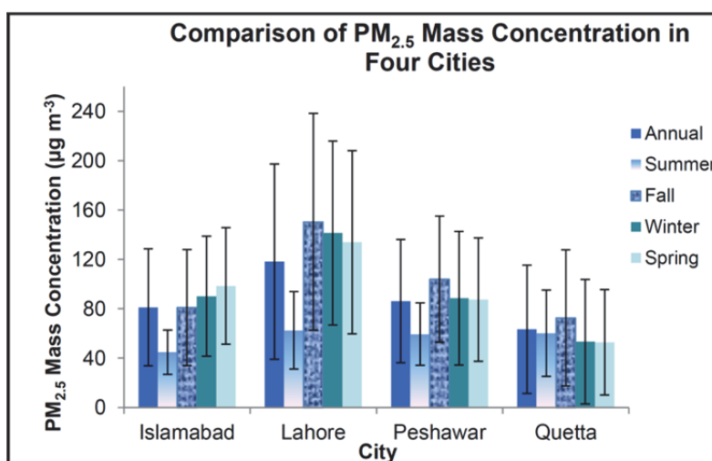
Fig. 2(b). Comparison of Annual and Seasonal Average \text{PM}_{2.5} Mass Concentration ( \mu\text{g}/\text{m}^3 ) in Islamabad, Lahore, Peshawar and Quetta during Summer 2007–Spring 2008 ( \pm 1 standard deviation is also shown in the figure).
